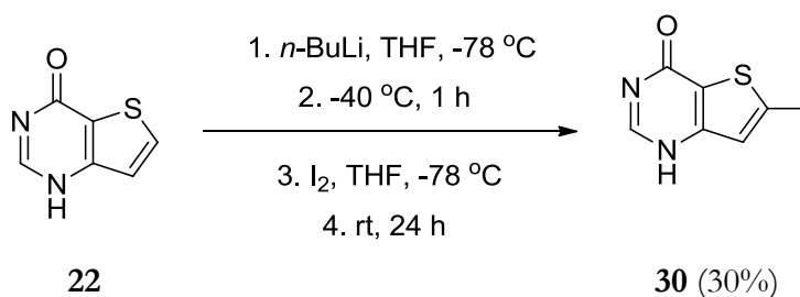
Scheme 18: Iodination of the Thieno[3,2- d ]pyrimidone 22
