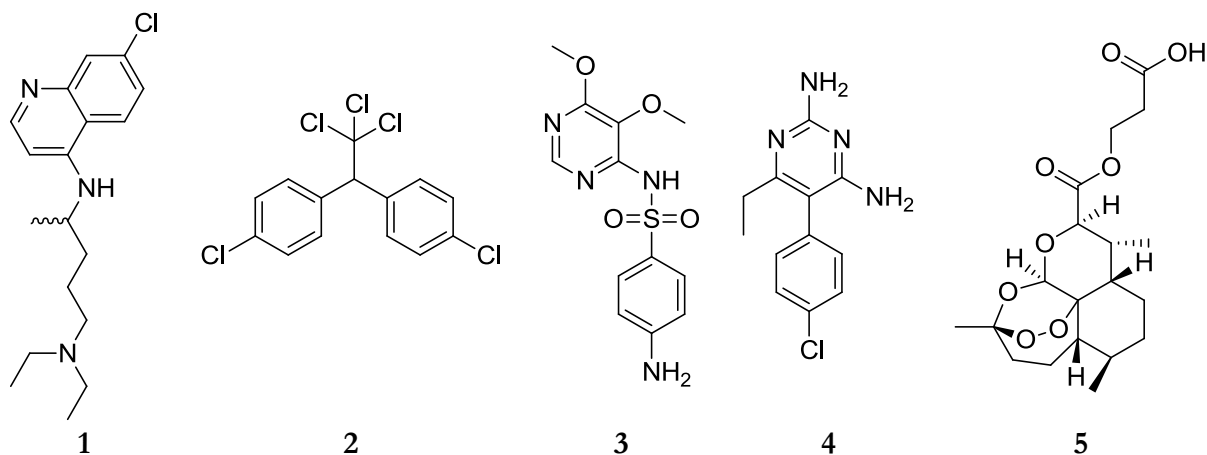
Figure 2: Treatments Used for the Treatment and Prophylaxis of Malaria (from left to right: Chloroquine, DDT, Sulfadoxine, Pyrimethamine, and Artesunate)
