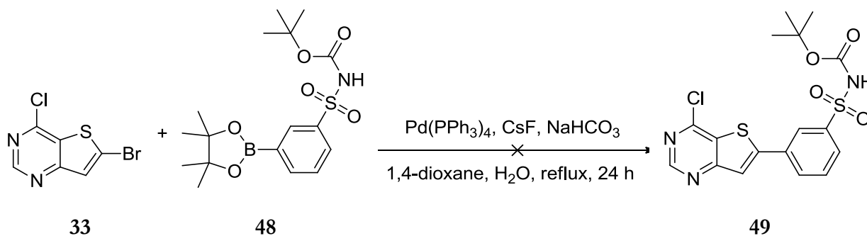
Scheme 31: Failed Suzuki Coupling of Boc -protected Sulfonamide 48
