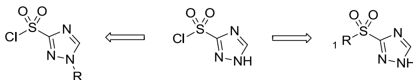
Figure 10: Possible Methods to Synthesise TCMDC 134395 ( 9 ) Analogues
