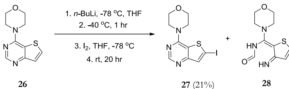
Scheme 16: Lithiation/Halogenation of the Morpholine Derivative 26
