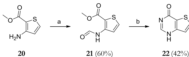
Scheme 12: Assembly of the Thieno[3,2- d ]pyrimidone 22 . Reagents and Conditions: a) NH 4 OAc, formic acid, reflux, 3 h; b) ammonium formate, formamide, reflux, 20 h.
