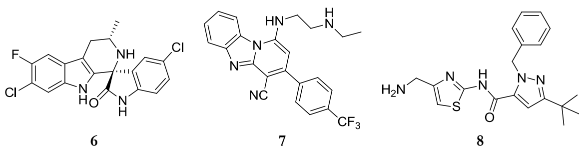
Figure 4: Three Promising Antimalarial Treatments in the Current Pipeline
