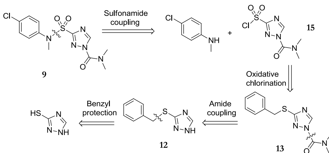
Scheme 1: Retrosynthesis of TCMDC 134395 ( 9 )
