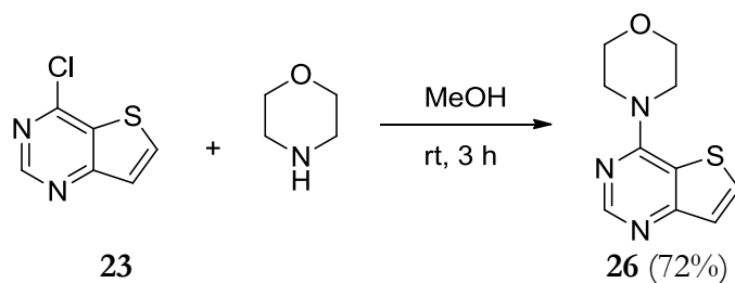
Scheme 15: Synthesis of Morpholine Derivative 26
