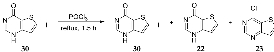
Scheme 19: Products from Chlorination of the Iodinated Thieno[3,2- d ]pyrimidone 30
