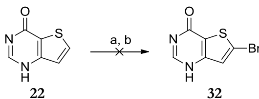
Scheme 21: Failed Bromination of the Thieno[3,2- d ]pyrimidone 22 . Reagents and Conditions: a) i) n -BuLi, THF, -78 °C, ii) -40 °C, 1 h, iii) Br 2 , -78 °C, iv) rt, 3 h; b) i) n -BuLi, THF, -78 °C, ii) -40 °C, 1 h, iii) CH 2 BrCH 2 Br, -78 °C, iv) rt, 3 h.
