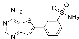
10 (TCMDC 135294) IC_{50} (3D7): 151 nM %Inhibition HepG2 (10 \mu M): 13
