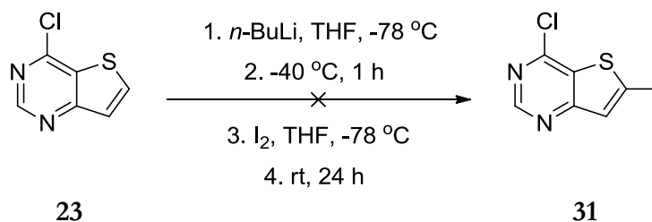
Scheme 20: Failed Iodination of the Chlorinated Thieno[3,2- d ]pyrimidine 23
