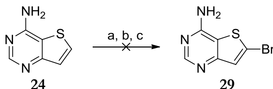
Scheme 17: Failed Halogenation of 24 . Reagents and Conditions: a) DMF, rt, 24 h; b) cat. H 2 SO 4 , CHCl 3 , rt, 24 h; c) Br 2 , 33% HBr/AcOH, Et 2 O, H 2 O, reflux, 6 h.
