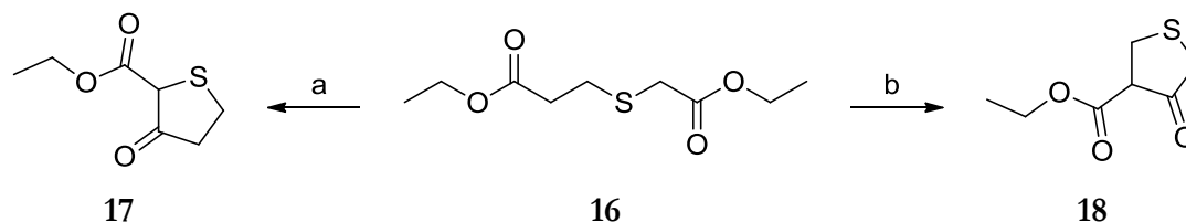
Scheme 10: The Kinetic (left) and Thermodynamic (right) Products of a Dieckmann Condensation on the Conjugate Addition Product 16 . Reagents and Conditions: a) NaOEt, EtOH, 0 °C, 6 h. b) NaOEt, PhMe, reflux, 6 h
