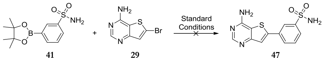
Scheme 29: Failed Synthesis of the Desired Suzuki Product 47
