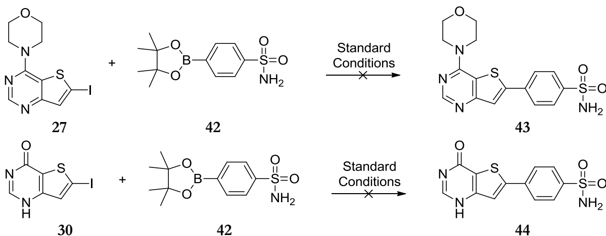
Scheme 27: Attempted Suzuki coupling of 30 and 42 , and of 27 and 42
